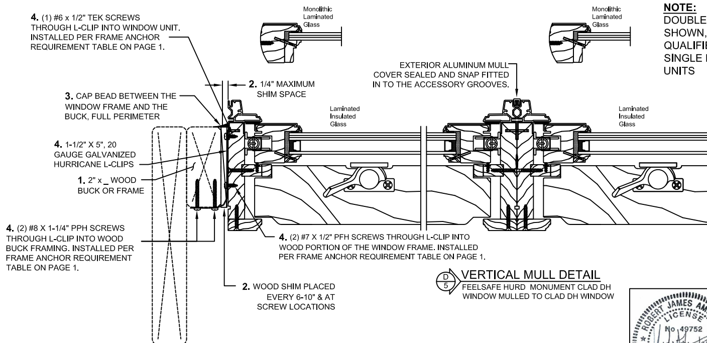
JAMB DETAIL FEELSAFE HURD MONUMENT CLAD DOUBLE HUNG WINDOW
