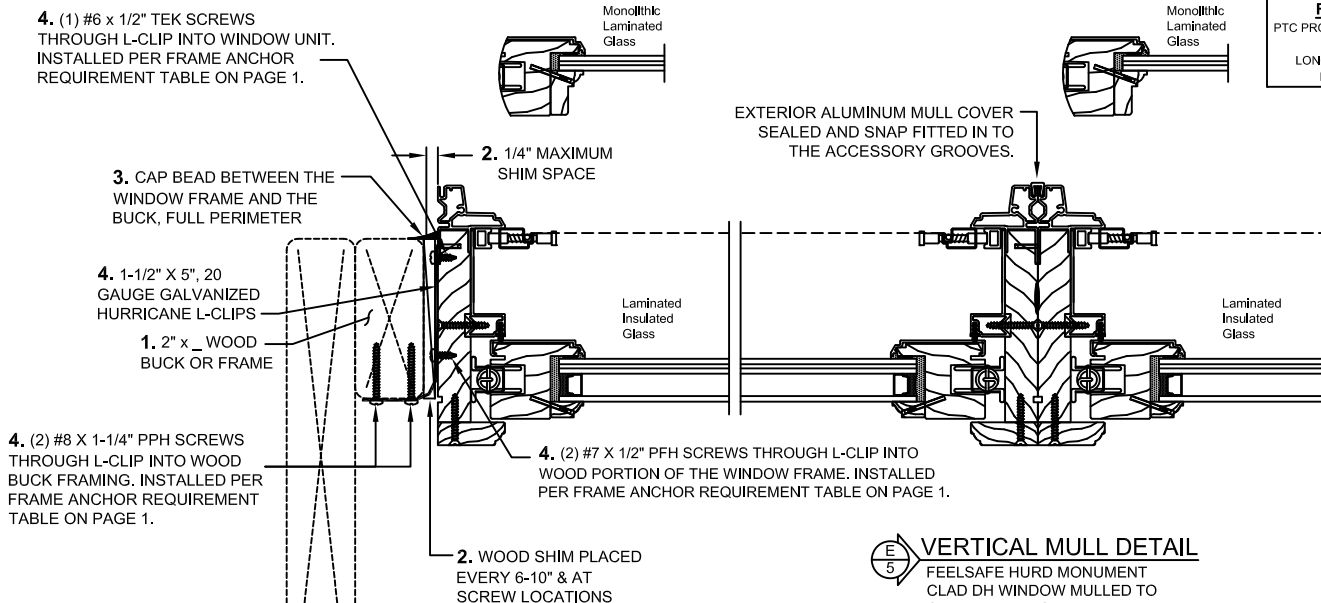
JAMB DETAIL FEELSAFE HURD MONUMENT CLAD DOUBLE HUNG WINDOW
